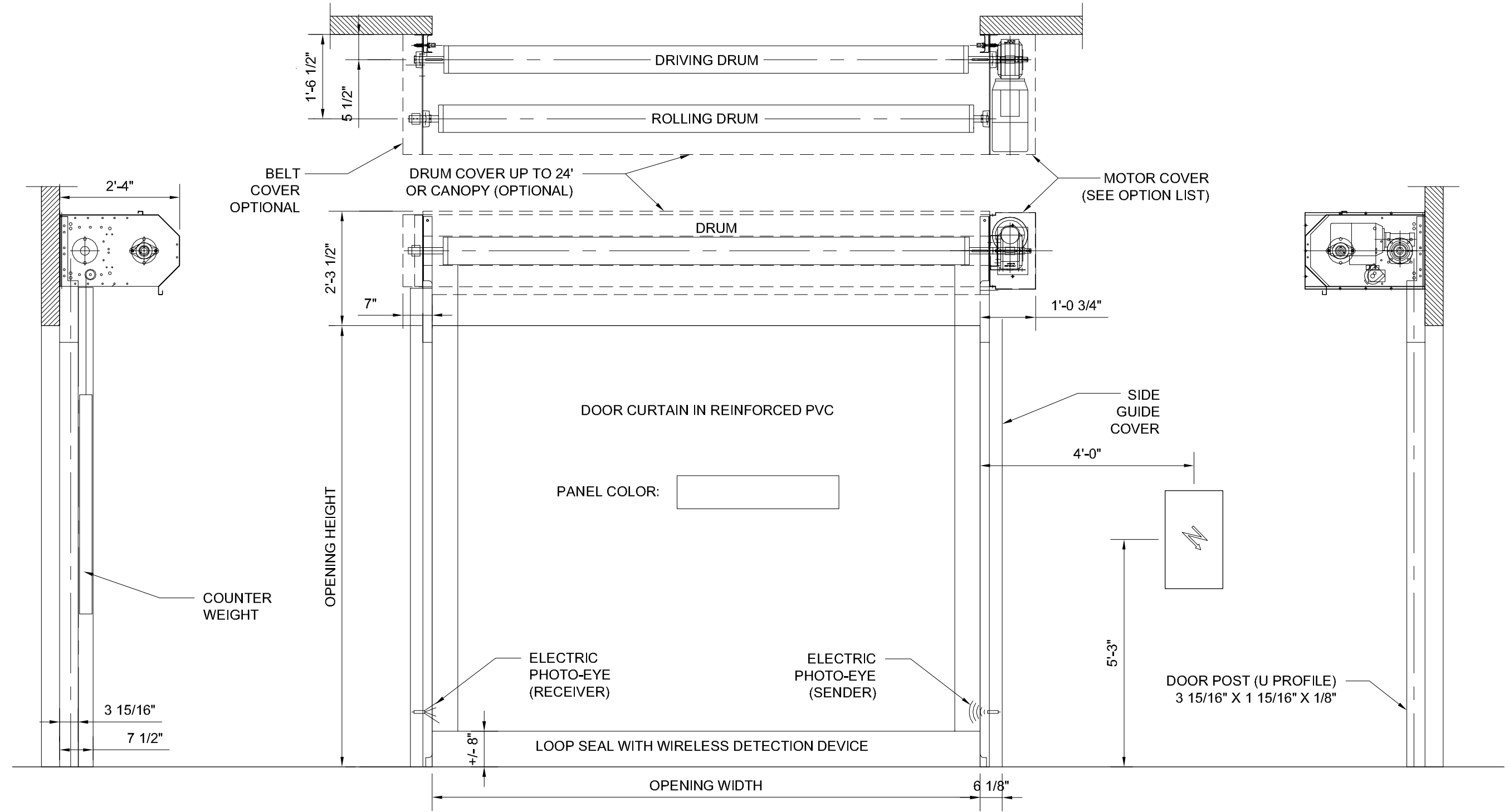
ELEVATION VIEW - LEFT
