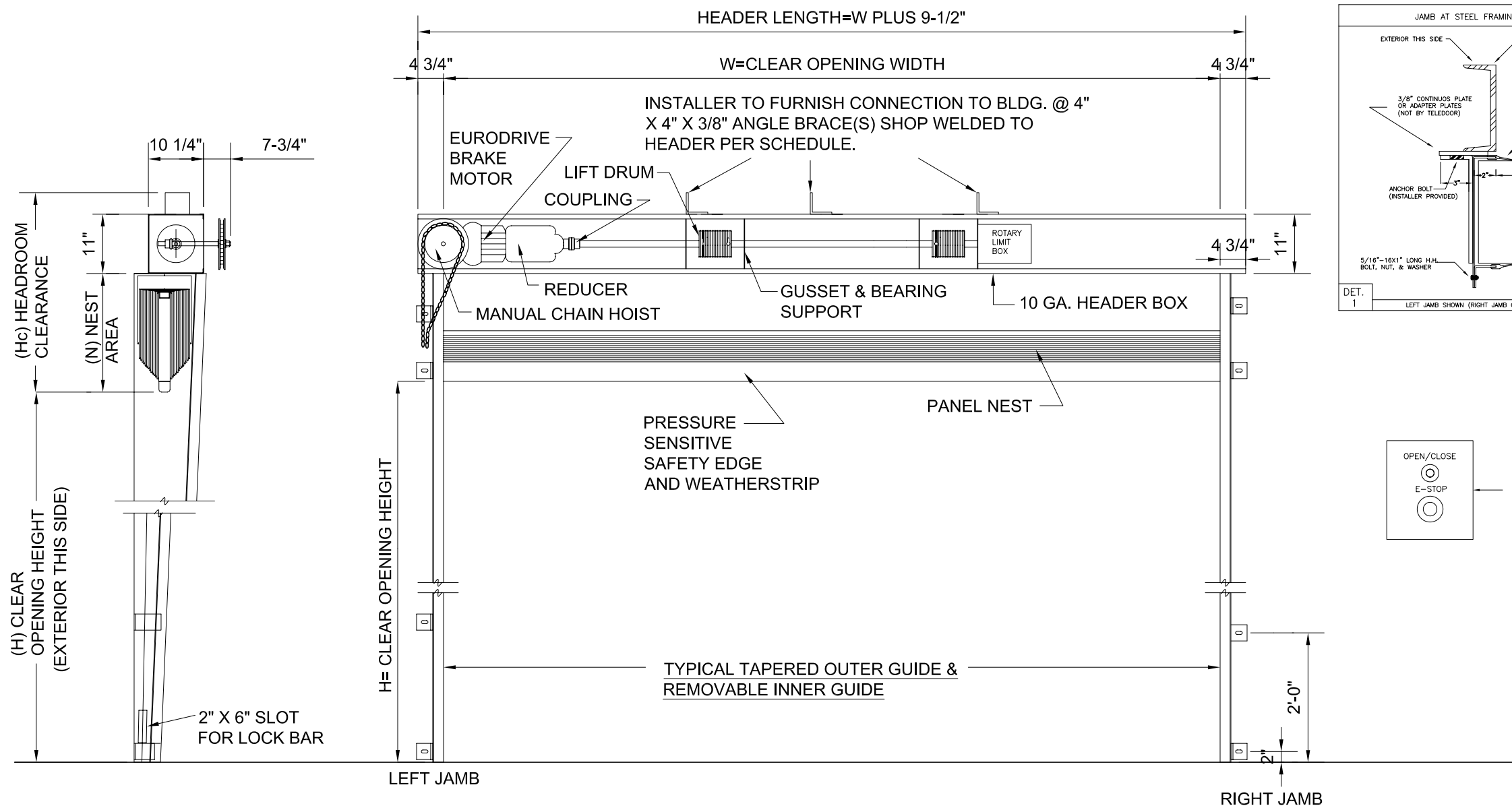
ELEVATION VIEW - LEFT
